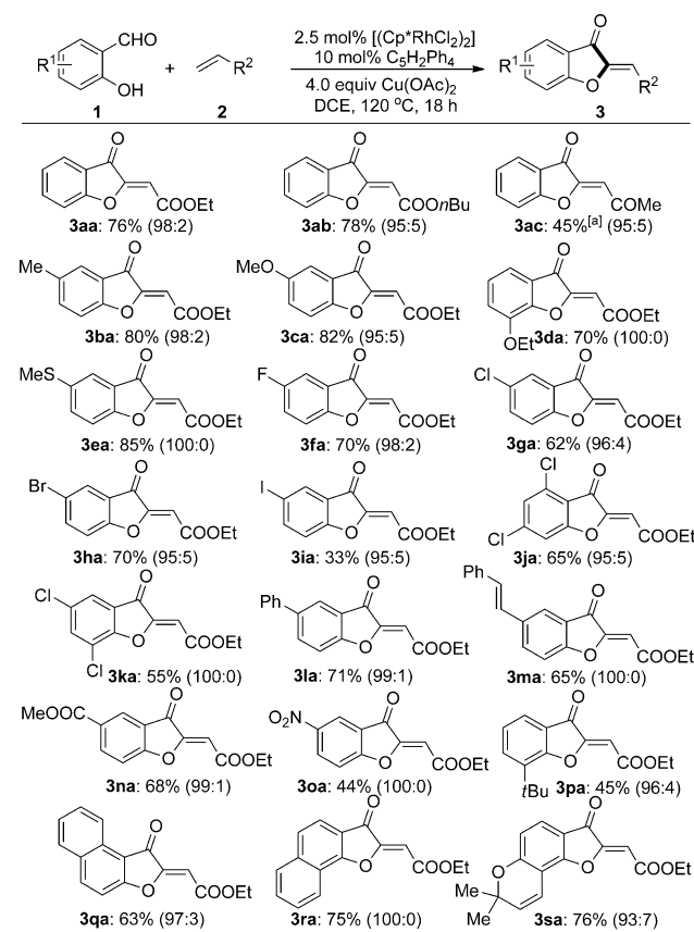
Scheme 2. \text{Rh}^{\text{III}} -catalyzed cyclization of salicylaldehydes and electron-deficient olefins. General reaction conditions: 1 (0.2 mmol), 2 (0.4 mmol), [(\text{Cp}^*\text{RhCl}_2)_2] (2.5 mol %), \text{C}_5\text{H}_2\text{Ph}_4 (10 mol %), \text{Cu}(\text{OAc})_2 (0.8 mmol), DCE (1.0 mL), 120 °C, 18 h, under Ar; values in parentheses indicate the Z/E ratios, which were determined by ^1\text{H} NMR analysis of the crude products. [a] Reaction temperature 90 °C.
